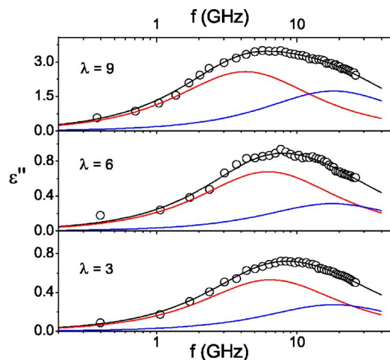
Figure 5. (Color online) Dielectric modes of water in hydrated Nafion 117 ( \lambda = 3, 6, and 9) at 25°C. The loss \epsilon''(f) relaxation distributions and their corresponding best fits, by two Debye processes, are shown. The faster process (high frequencies) corresponds to bulklike water and the slower process (lower frequencies) to loosely bound water.
