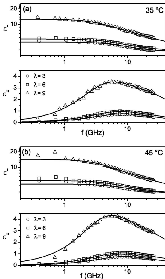
Figure A-3. Water relaxations for Nafion 117 with \lambda = 3, 6, and 9 at two higher temperatures: (a) 35^\circ\text{C} and (b) 45^\circ\text{C} . In all cases, fits are by two \epsilon''(\omega) Debye peaks whose peak frequencies ( f_{\text{max}}^{-1} = 2\pi\tau_{\text{max}} ) are shown in Fig. 7.
